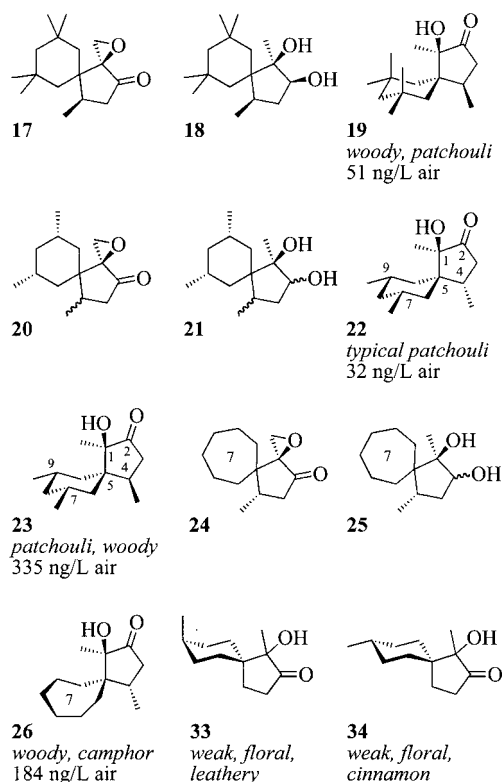
Figure 3. Overview of the structures of the synthesized analogous ketols 19 , 22 , 23 , 26 , 33 , and 34 with the respective intermediates 17 , 18 , 20 , 21 , 24 , and 25 .
