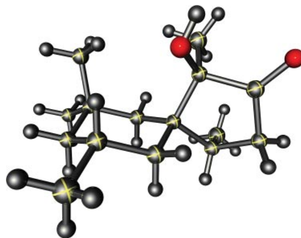
Figure 2. X-ray crystal structure of (1 R *,4 S *,5 S *,9 R *)-1-hydroxy-1,4,7,7,9-pentamethylspiro[4.5]decan-2-one ( 15 ) with thermal ellipsoids at the 50% probability level.
