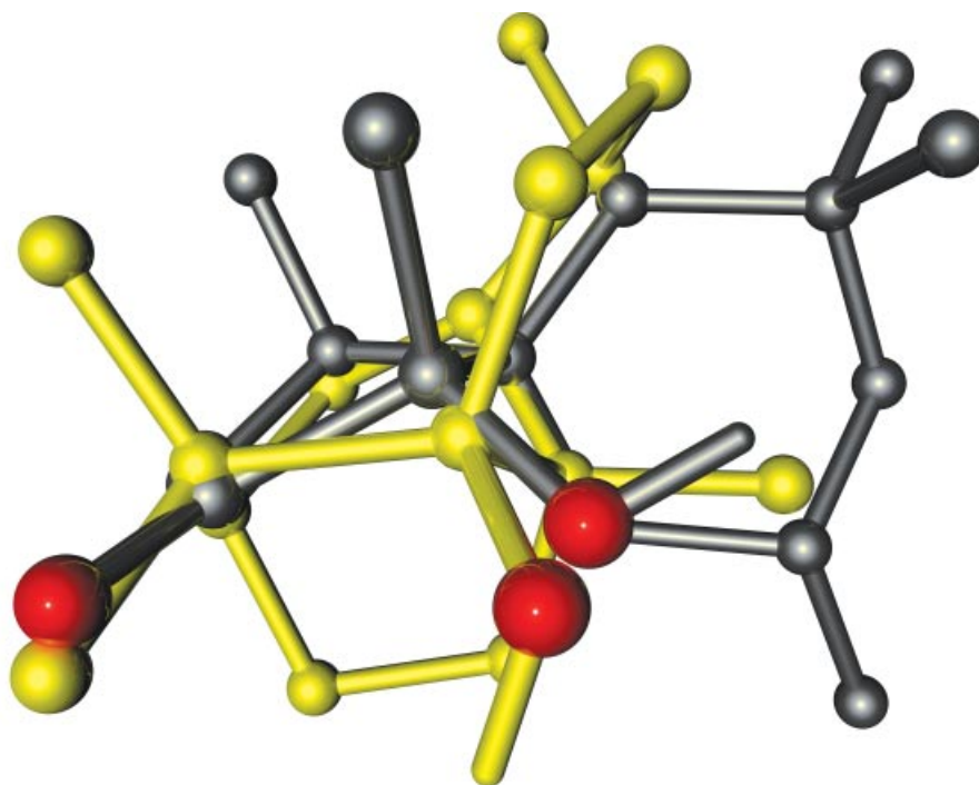
Figure 6. Superposition analysis of (+)-(1 S ,4 R ,5 R ,9 S )-1-hydroxy-1,4,7,7,9-pentamethylspiro[4.5]decan-2-one ( 38 , silver) and (–)-patchoulol ( 3 , gold).
