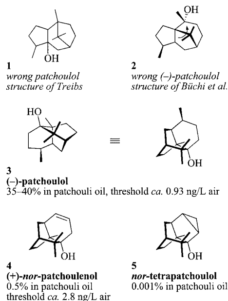
Figure 1. The naturally occurring patchouli odorants (–)-patchoulol (3), (+)-nor-patchoulol (4), and nor-tetrapatchoulol (5).
