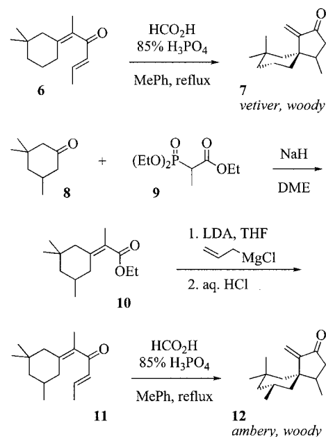
Scheme 1. Our synthetic route to novel spirocyclic vetiver odorants by Nazarov cyclization on the example of 4,7,7,9-tetramethyl-1-methylenespiro[4.5]decan-2-one (12) and 4,7,7-trimethyl-1-methylenespiro[4.5]decan-2-one (7), the most typical vetiver odorant synthesized.
