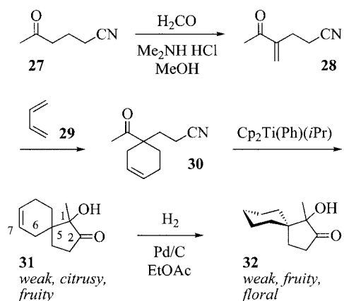
Scheme 3. Synthesis of the parent ketol 1-hydroxy-1-methylspiro[4.5]decan-2-one ( 32 ) by reductive intramolecular cyclization with the titanocene(III) complex \text{Cp}_2\text{Ti}(\text{Ph})(i\text{Pr}) .
