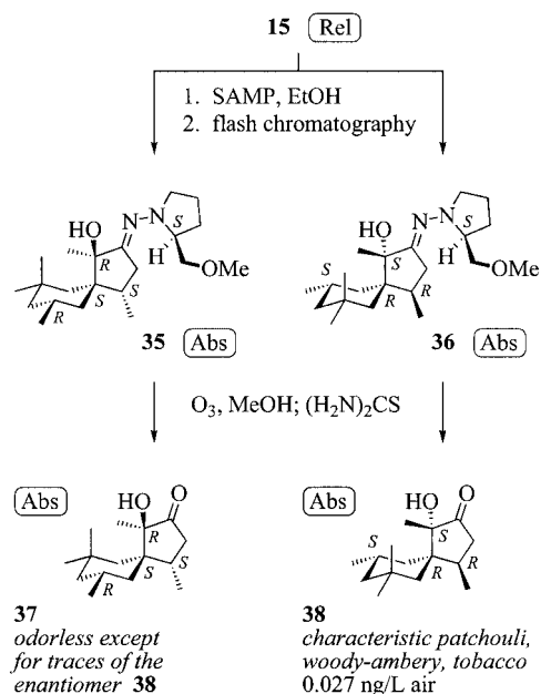
Scheme 4. Separation of the enantiomers of (1 R *,4 S *,5 S *,9 R *)-1-hydroxy-1,4,7,9-pentamethylspiro[4.5]decan-2-one ( 15 ) via their SAMP hydrazones 35 and 36 .
