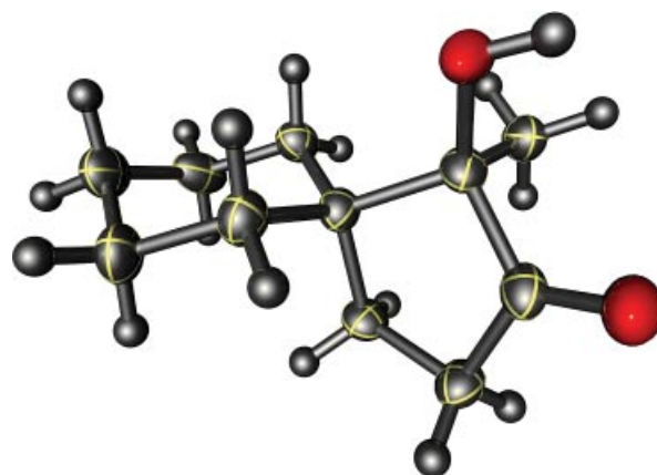
Figure 4. X-ray crystal structure of 1-hydroxy-1-methylspiro[4.5]decan-2-one ( 32 ) with thermal ellipsoids at the 50% probability level.
