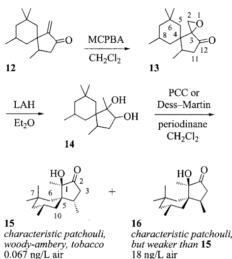
Scheme 2. Synthesis of the new high-impact patchouli odorant (1 R *,4 S *,5 S *,9 R *)-1-hydroxy-1,4,7,7,9-pentamethylspiro[4.5]decan-2-one ( 15 ) by epoxidation/LAH reduction and subsequent oxidation of 4,7,7,9-tetramethyl-1-methylenespiro[4.5]decan-2-one ( 12 ).
