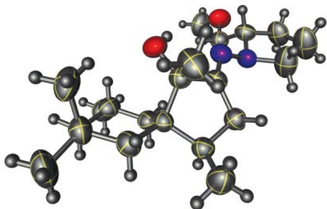
Figure 5. X-ray crystal structure of (+)-(1 S ,4 R ,5 R ,9 S ,2' S )-1-hydroxy-1,4,7,7,9-pentamethylspiro[4.5]decan-2-one 1'-amino-2'-methoxymethylpyrrolidine hydrazone ( 36 ) with thermal ellipsoids at the 50% probability level.
